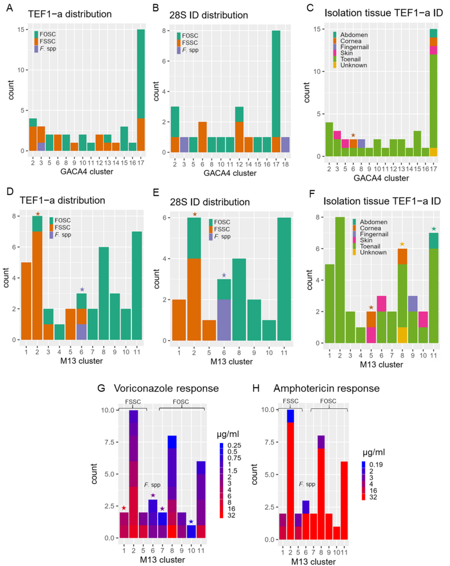
Figure 2. (GACA)4 and M13 association with several epidemiological variables. Cluster associations with the sequencing-based identification of the isolates for (GACA) 4 (A, B) and M13 (D, E). Associations with the isolation tissue (C, F) for each marker clusters and associations between M13 and the response to antifungal compounds (G, H). M13 clusters 1 to 5 are enriched with isolates classified as FSSC, cluster 6 with Fusarium spp, and clusters 7 to 11 with FO SC. Significant hypergeometric values (p-adjusted <0.001) reported for category-mixed clusters indicating the significant category with the same color as in the histogram.
