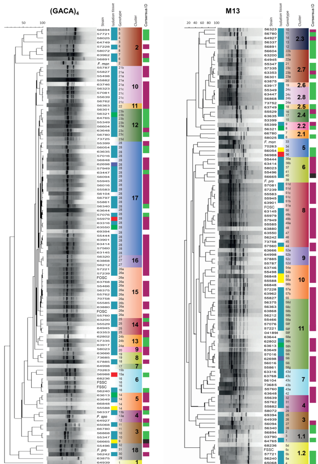
Figure 1. (GACA) 4 and M13 dendrograms obtained by the UPGMA method using the Pearson correlation. The first column of each dendrogram correspond to the strain number. Several refence strains were included and abbreviated as FSSC ( F. solani (Mart.) Sacc.), FOSSC ( F. oxysporum Smith & Swingle), F. mon ( F. moniliforme J. Sheld. 1904), F. pro ( F. proliferatum (Matsush.) Nirenberg 1976), and F. spo ( F. sporotrichioides Sherb. 1915). The second column refers to the isolation tissue (blue: toenails, green: fingernails, purple: abdomen, red: cornea, and yellow: skin). The third column shows the genotypes classification with their number and clusters (differentiated by color and number). The last column refers to the consensus-sequencing identification (green: FSSC, purple: FOSSC, and black: Fusarium incarnatum ).
